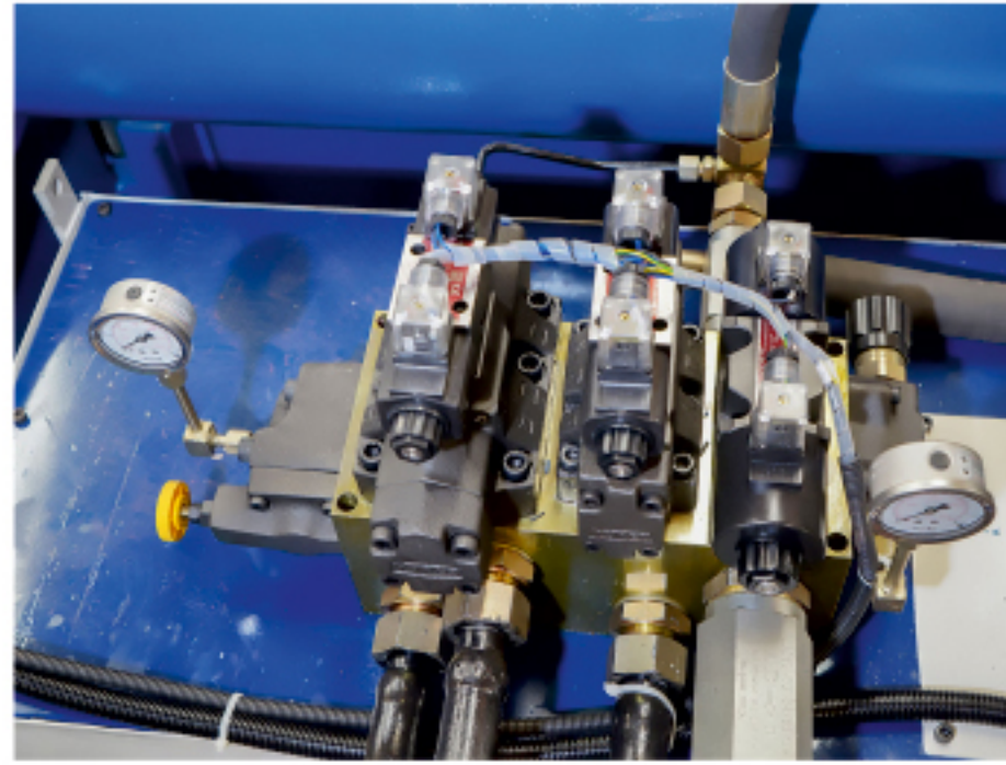
Bosch rexroth /yuken make hydraulic system
