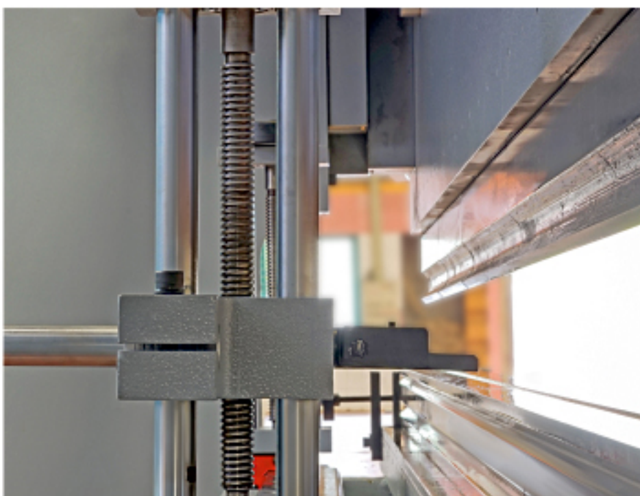
Back Gauge Fingers
