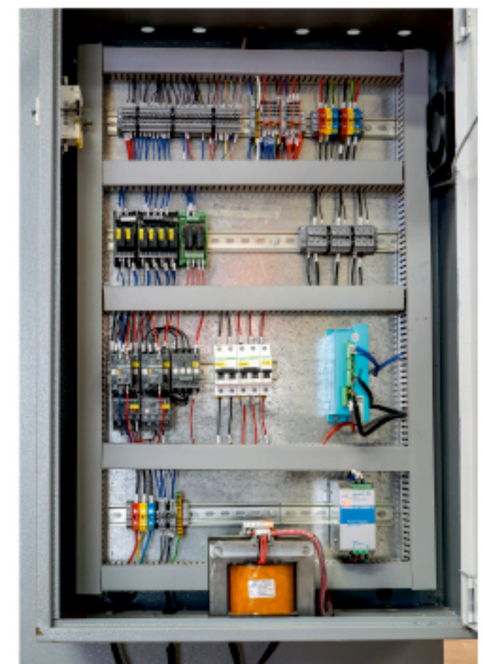
Electric Panel Schneider
