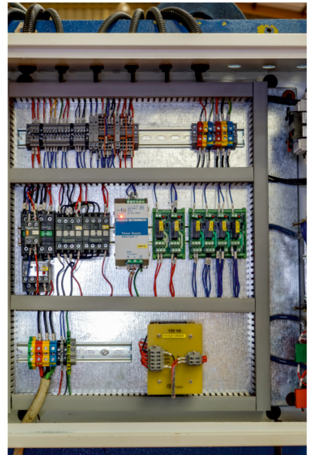
Electrical panel in-house make
