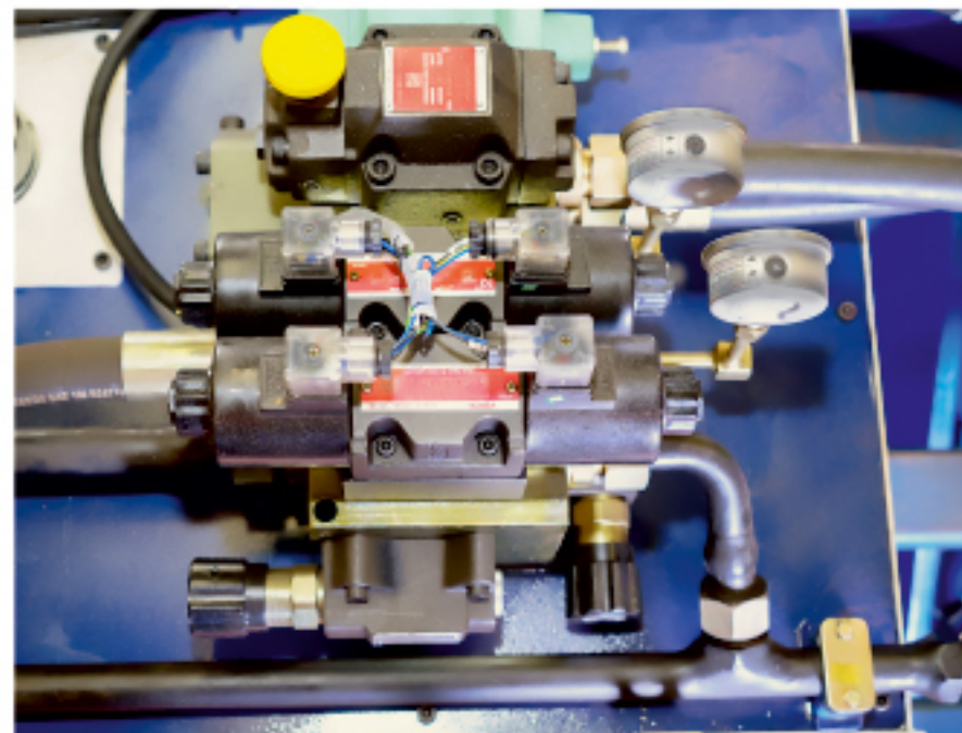
Bosch Rexroth / Yuken Hydraulic system
